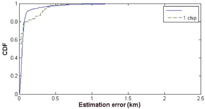
Fig. 6. CDF of estimation error for suburban ITU Vehicular A.
