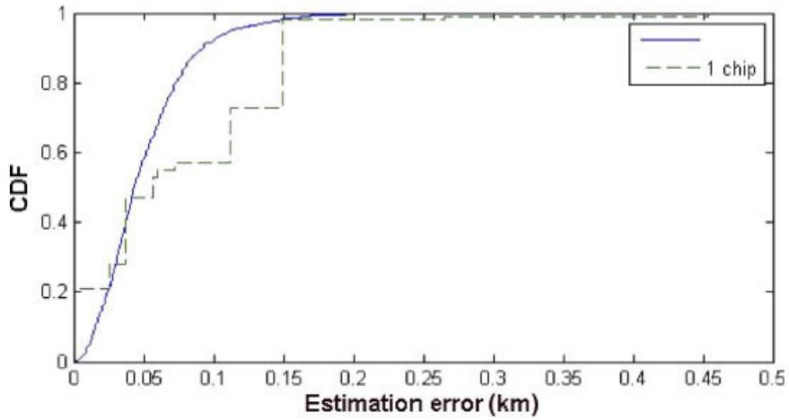
Fig. 5. CDF of estimation error for suburban ATDMA model.
