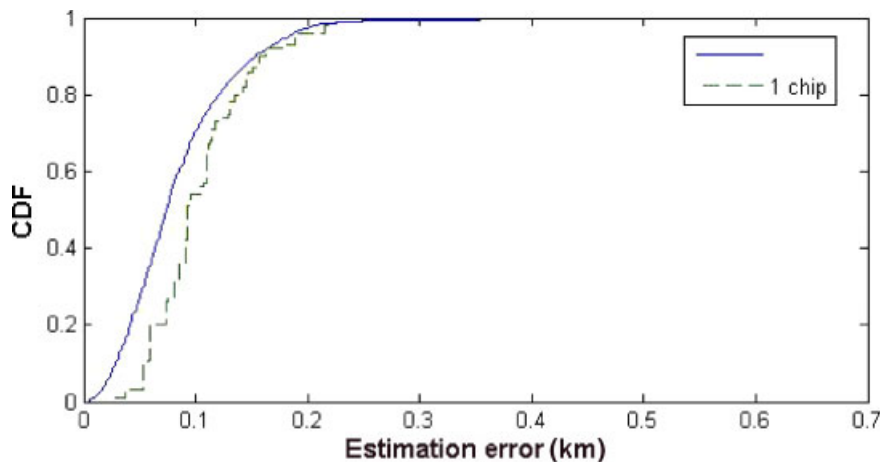
Fig. 4. CDF of estimation error for suburban CODIT model.
