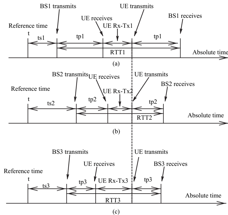
Fig. 1. Base stations and mobile station transmit and receive timing diagrams for (a) BS1, (b) BS2, and (c) BS3.
