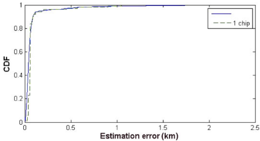
Fig. 7. CDF of estimation error for suburban ITU Vehicular B.
