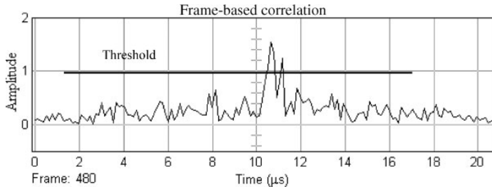
Fig. 2. Correlation of the incoming signal with the locally generated long code.
