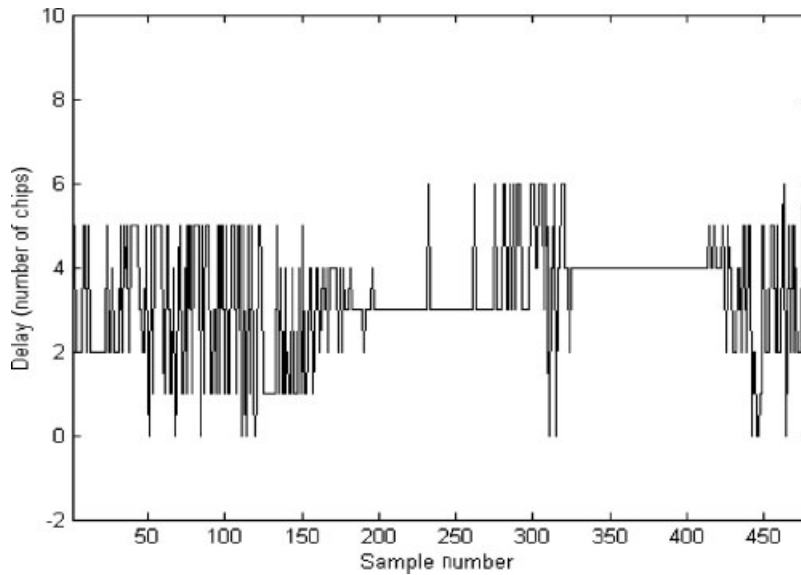
Fig. 3. Chip delay versus sample number for CODIT Macro model.
