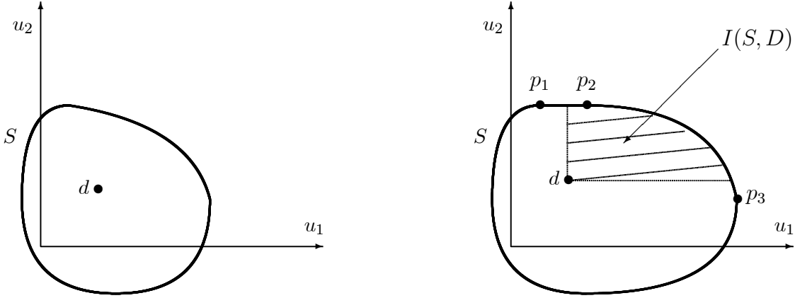
Figure 1: On the left: a strictly d -comprehensive bargaining problem. On the right: a weakly d -comprehensive bargaining problem, the individually rational set, the Pareto set (part of the north-east boundary between p_2 and p_3 ) and the weak Pareto set (part of the north-east boundary between p_1 and p_3 ).
