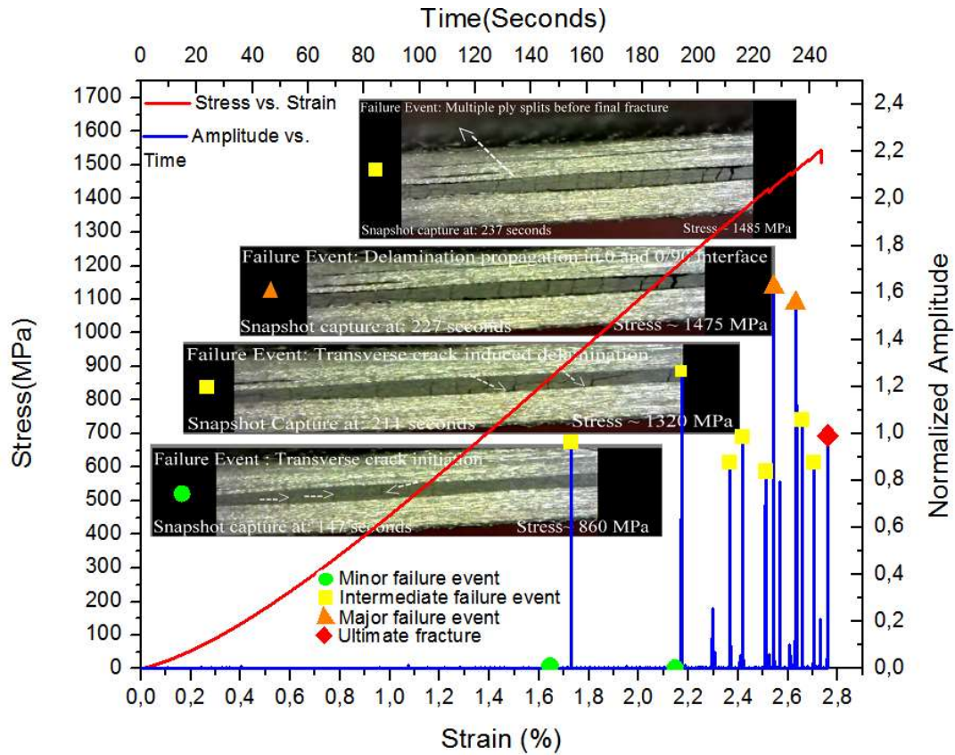
Figure 5: Stress vs. Strain , Amplitude vs. Time plots for (0_5/90)_s laminates and snapshot captures from video 3.
