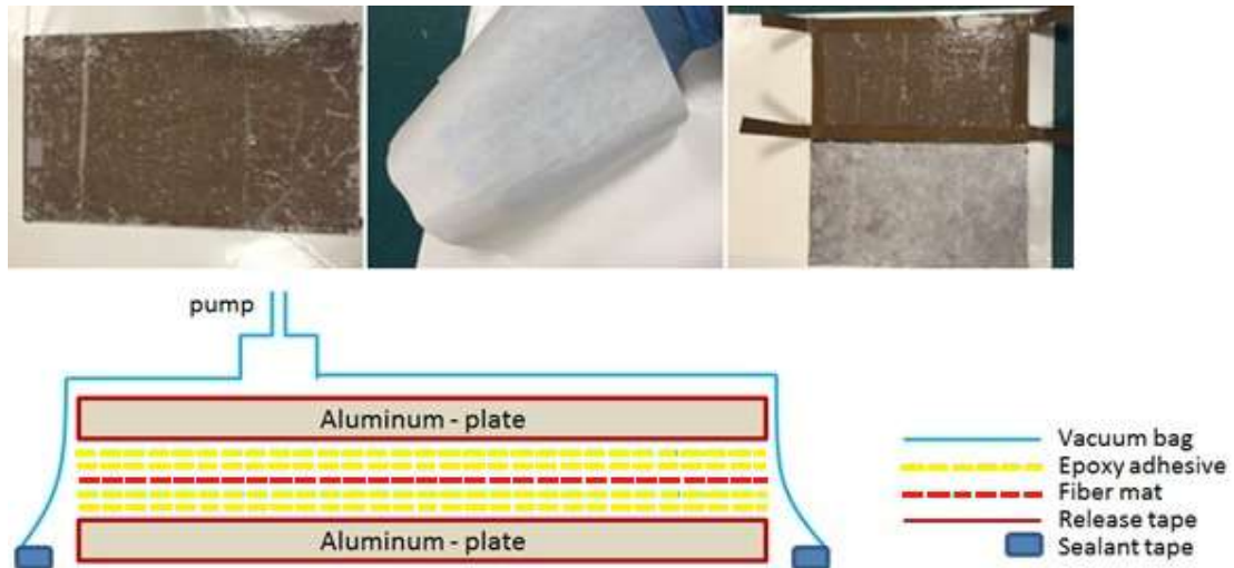
Figure 1: A view from adhesive film casting process
