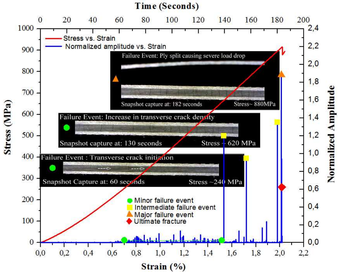
Figure 4: Stress vs. Strain , Amplitude vs. Time plots for (0_3/90_3)_s laminates and snapshot captures from video 2.
