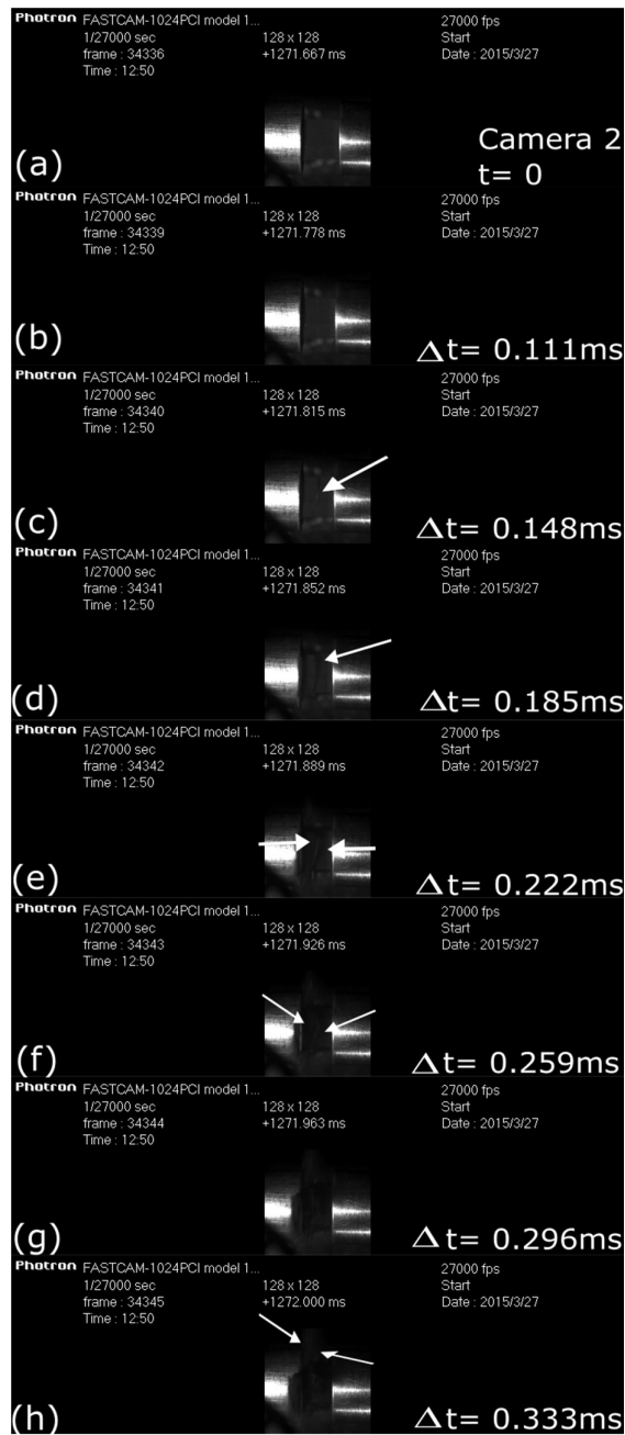
Figure 7. Progressive damage of nanofiber interlayered (0/90)_{25s} composites with applied load in thickness direction at strain rate of 2600 \text{ s}^{-1} , high speed photography images are taken from mounted Camera 2 . ( t=0 , time of impact)
