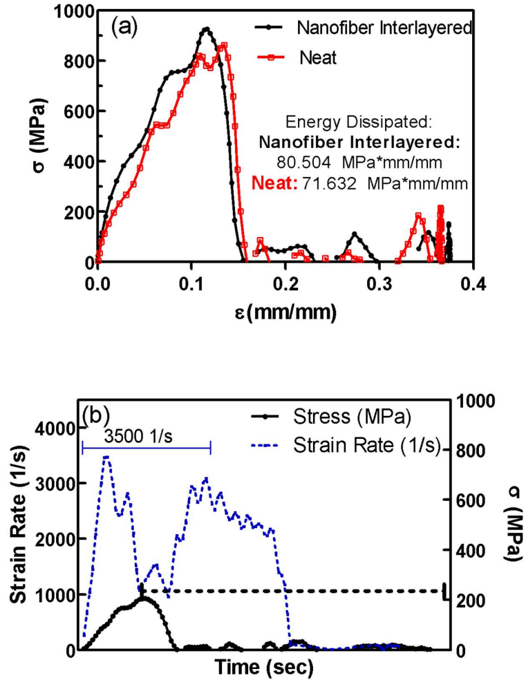
Figure 5: (a) Stress–strain ( \sigma – \epsilon ) and (b) Strain rate and stress versus time plots of neat (0/90)_{25s} and nanofiber interlayered (0/90/I)_{25s} laminates through thickness loading at strain rate of 3500 \text{ s}^{-1}
