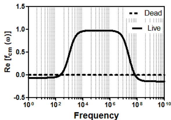
Figure 1. Characterization of the live and dead U937 monocytes. The Re[f_{cm}(w)] vs. frequency (Hz) data is obtained using the dielectric properties of the live (continuous line) and dead (dashed line) monocytes.
