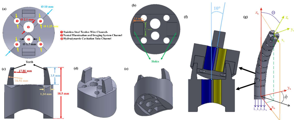
Figure 1. (a) The outer and channel diameters of bendable spacer in X axis; the placement of components, (b) dimensions of the holes, (c) length of the part, (d) and (e) perspective view of the part, (f) bending mechanism of a flexible pair, (g) the relationship between actuation space ( L ) and joint space ( \theta, \phi )
