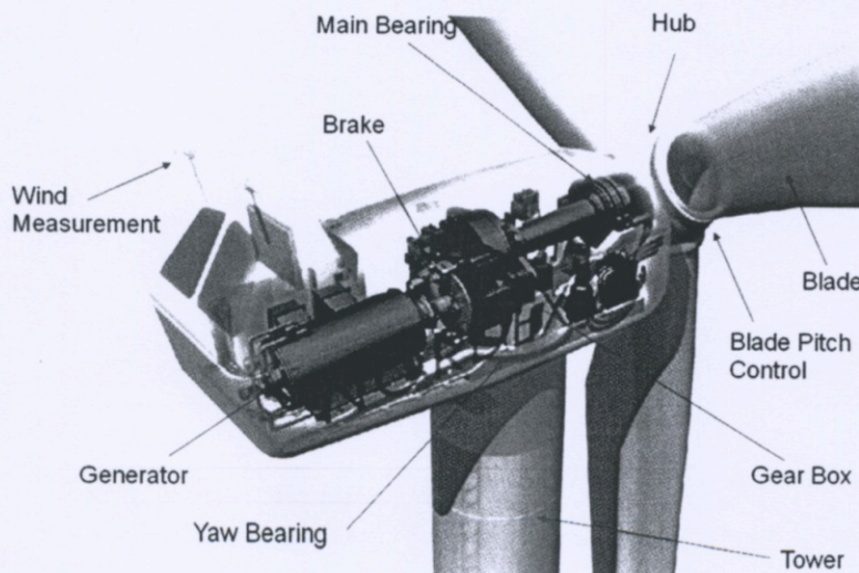
Figure 2. Components of a typical wind turbine as illustrated on NORDEX N80.
