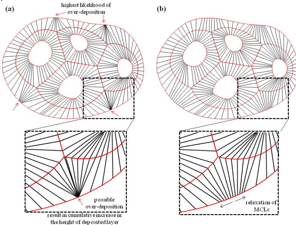
Fig. 5: MCL Relaxation Technique to alleviate over-deposition
