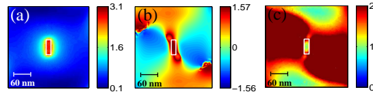
Fig. 3. (a) |\mathbf{E}|^2 , (b) |\Delta\phi| and (c) |\mathbf{E}_y| / |\mathbf{E}_x| for \alpha_{pol} = 68^\circ for G_h = 20 nm and G_v = 60.5 nm.
