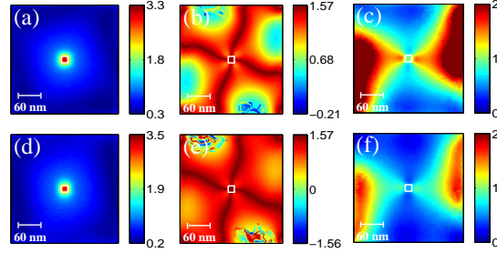
Fig. 2. First and second rows are for circularly and elliptically polarized illuminations, respectively. (a) and (d) |\mathbf{E}|^2 , (b) and (e) |\Delta\phi| , (c) and (f) |\mathbf{E}_y| / |\mathbf{E}_x| at z = 20 nm.
