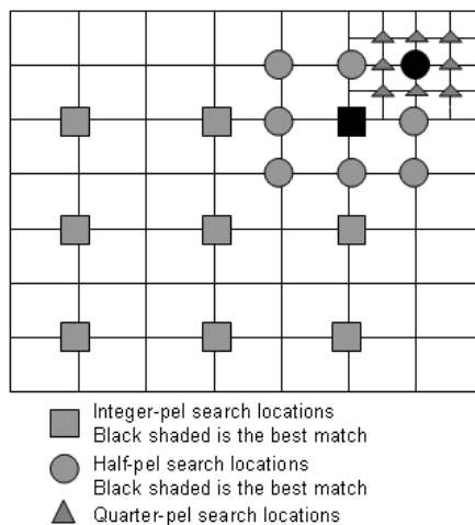
Figure 3.1 Half-Pixel and Quarter-Pixel Search Locations
