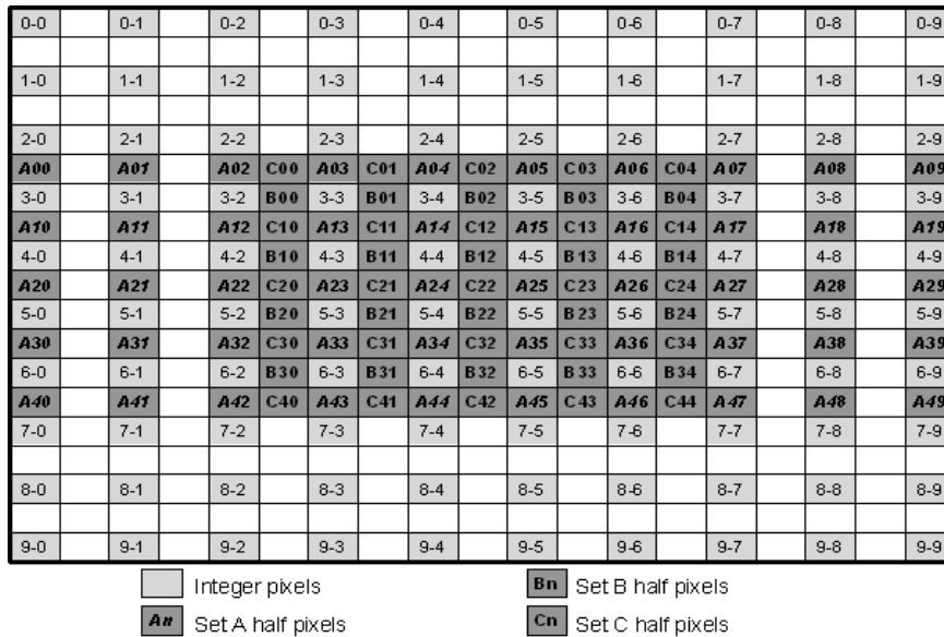
Figure 2.4 Half-Pixel Interpolation Flow
