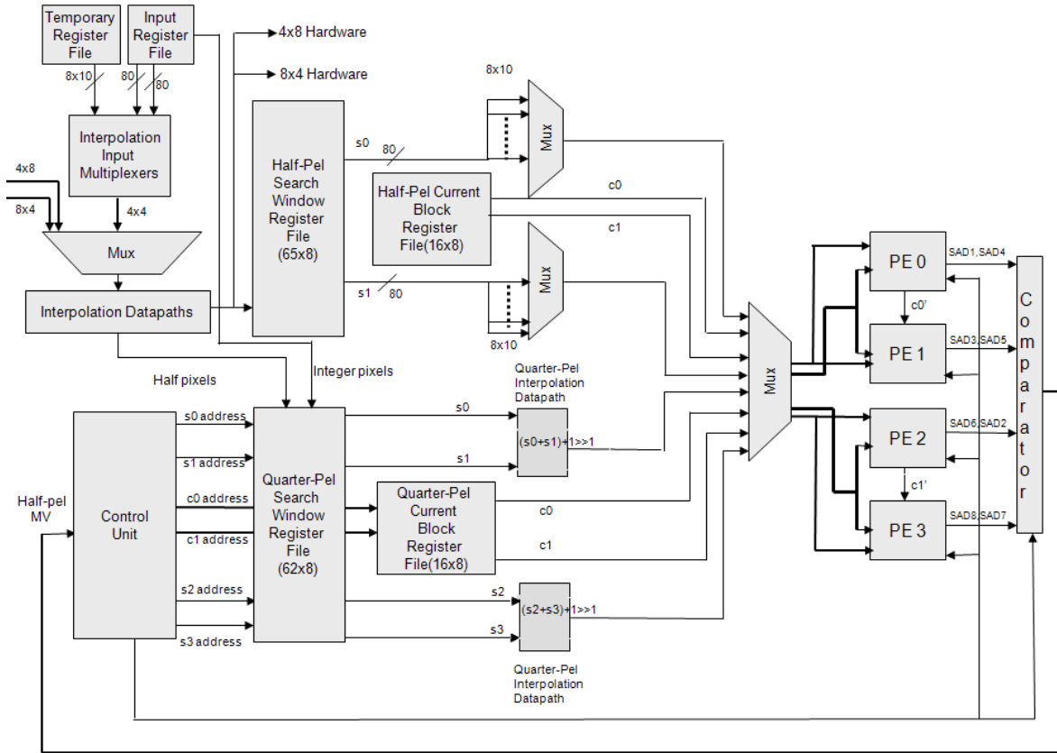
Figure 4.3 Proposed Sub-Pixel Accurate Motion Estimation Hardware for 4x4 Block Size
