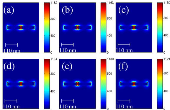
Figure 5. Total |E|^2 distribution in the presence of nano-antennas. The fields are plotted on the x-y cut plane for: (a) \alpha = 5^\circ , (b) \alpha = 15^\circ , (c) \alpha = 30^\circ , (d) \alpha = 45^\circ , (e) \alpha = 60^\circ , and (f) \alpha = 75^\circ .
