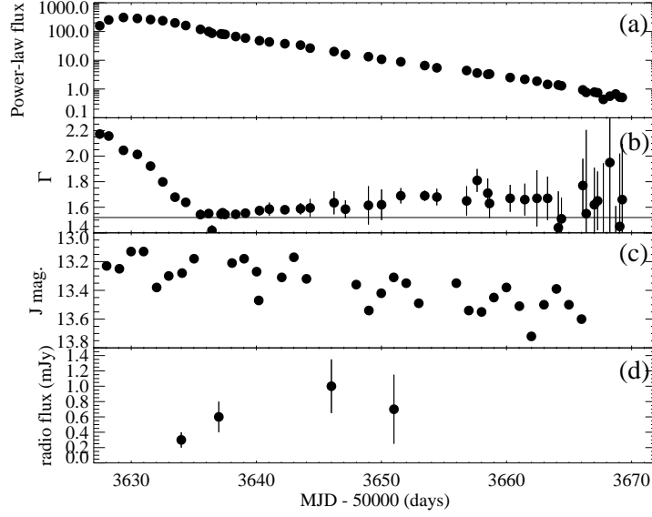
Figure 2: 2005 outburst decay of GRO J1655-40; the evolution of (a) the power law flux in 3-25 keV band in units of 10^{-11} ergs \text{cm}^{-2} \text{s}^{-1} , (b) the photon index, (c) the J-band magnitude, (d) the radio flux
