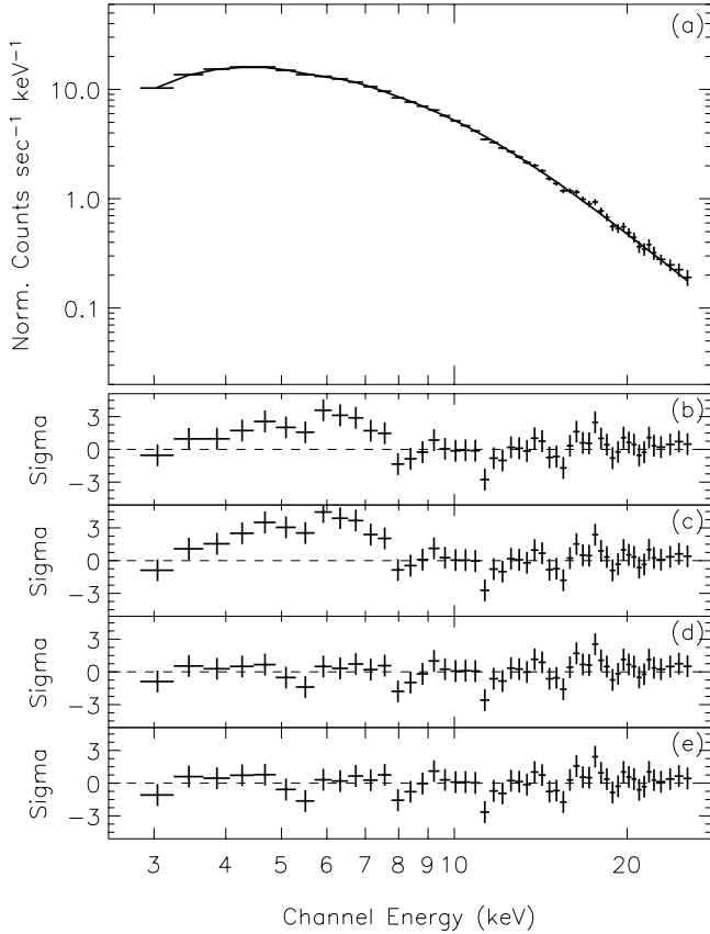
FIG. 7.—Representative spectral fit of a PCA observation during the early hard state of XTE J1908+094 (on day 62). (a) Count spectrum and the best-fit multicolor disk blackbody (MCD) + broad line + power law model all attenuated by the interstellar absorption ( solid line ). (b) Residuals of the best-fit single power-law model ( \chi^2_\nu = 1.87 ). (c) Residuals of the best-fit MCD + power law model ( \chi^2_\nu = 2.66 ). (d) Residuals of the best-fit broad line + power law model ( \chi^2_\nu = 0.88 ). (e) Residuals of the best-fit MCD + broad line + power law model ( \chi^2_\nu = 0.87 ).
