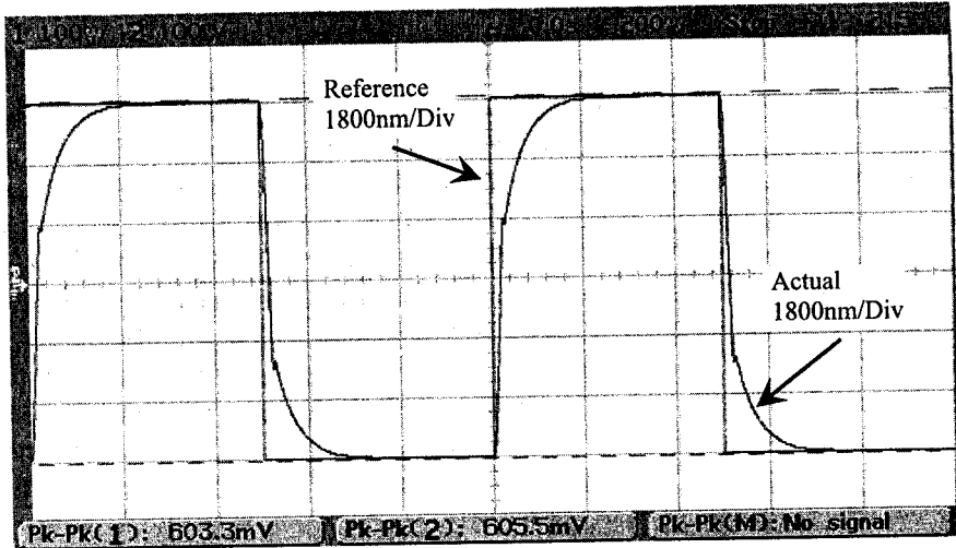
Fig. 9. Analog circuit tracking experiment for 10.8\mu\text{m} peak to peak reference sinus of 1Hz
