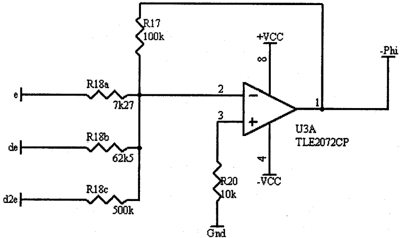
Fig. 3. Calculation of \phi from previously found variables; e , \dot{e} and \ddot{e}
