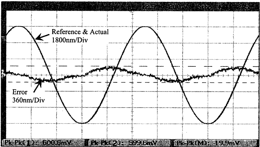
Fig. 8. Analog circuit tracking experiment for 10.8\mu\text{m} peak to peak reference sinus of 1Hz
