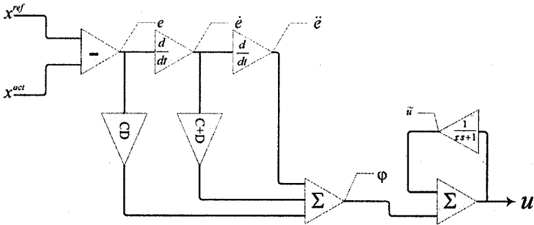
Fig. 1. Draft analog circuit scheme to calculate the control.
