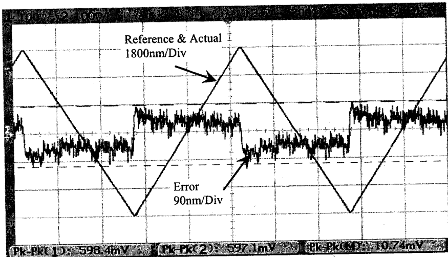
Fig. 10. Analog circuit tracking experiment for 4.5\mu\text{m} peak to peak reference triangular wave
