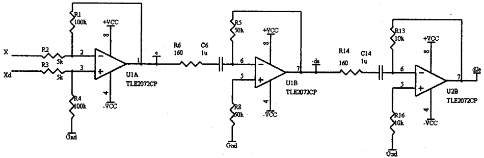
Fig. 2. Preparation of the necessary variables ( e , \dot{e} and \ddot{e} ) from the desired and actual inputs; x_d and x
