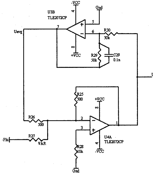
Fig. 4. Calculation of u = \tilde{u} + K \cdot \varphi where \tilde{u} is found through the first order filtering of the control and K is obtained by the tuning of the resistor R_{27} since
