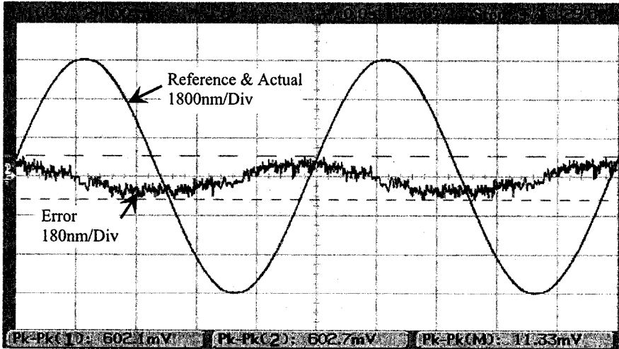
Fig. 7. DSP tracking experiment for 10.8\mu\text{m} peak to peak 1Hz sinusoidal reference
