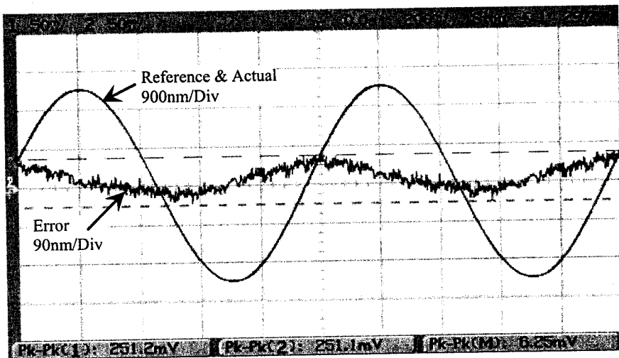
Fig. 6. DSP tracking experiment for 4.5\mu\text{m} peak to peak 1Hz sinusoidal reference
