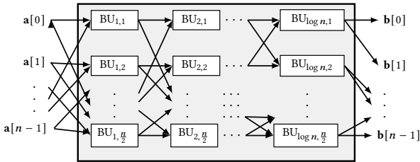
Figure 2: Loop unrolling, as illustrated for iterative \text{NTT}_n , requires \log n \cdot (n/2) BUs.
