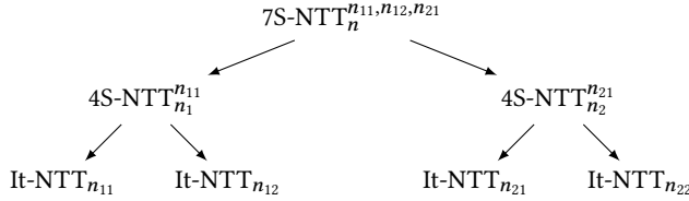
Figure 1: Illustration of seven-step NTT with recursive four-step NTTs. 7S-NTT _n^{n_{11}, n_{12}, n_{21}} denotes seven-step NTT with 4-D decomposition n = n_{11} \times n_{12} \times n_{21} \times n_{22} . 4S-NTT _n^{n_{11}} denotes four-step NTT where n = n_{11} \times n_{21} while It-NTT denotes the iterative NTT. Twiddle multiplications are not visualized.
