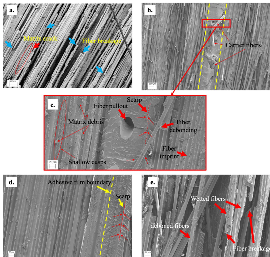
FIGURE 5 | SEM image of fracture surface after transverse tensile test for (a) REF and (b-e) ALE samples.
