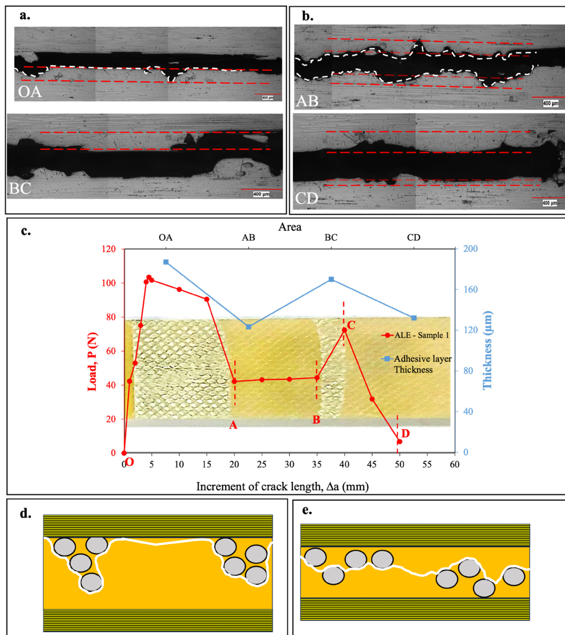
FIGURE 11 | Correlation between fracture mechanism and carrier fibers positioning. Cross-sectional microscopy images represent (a) thin-layer cohesive failure, (b) cohesive failure, (c) load and thickness variation curves with crack length, and schematic representation of crack growth and thickness variation for (d) thin-layer cohesive failure, and (e) cohesive failure.
