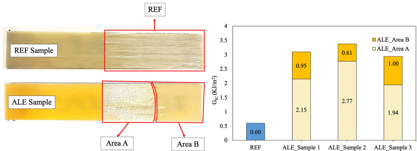
FIGURE 8 | Representative fracture surfaces and G_{IC} values of the REF and three ALE samples with portions of area A (whitish) and area B (yellowish).
