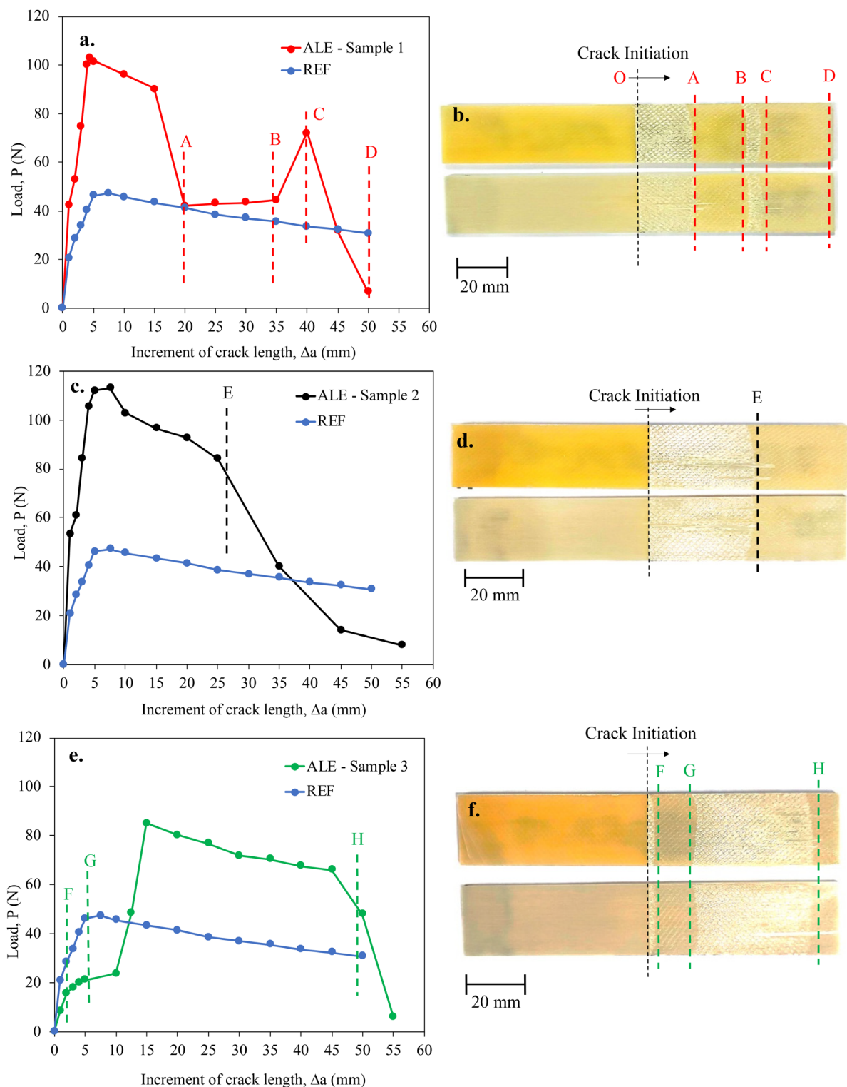
FIGURE 7 | Correlation between load-crack length curves (a, c, and e) and fracture surface images (b, d, and f) for ALE samples 1, 2, and 3, respectively under Mode-I fracture tests.
