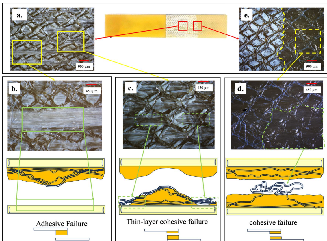
FIGURE 9 | Stereo-microscopy images and attributed fracture mechanisms for DCB samples under Mode-I fracture tests for ALE samples exemplifying for (a) ALE sample 2, (b) whitish region with adhesive failure and (c) thin-layer cohesive failure: and for yellowish region (d) cohesive failure mechanisms and (e) boundary between two distinct fracture areas.
