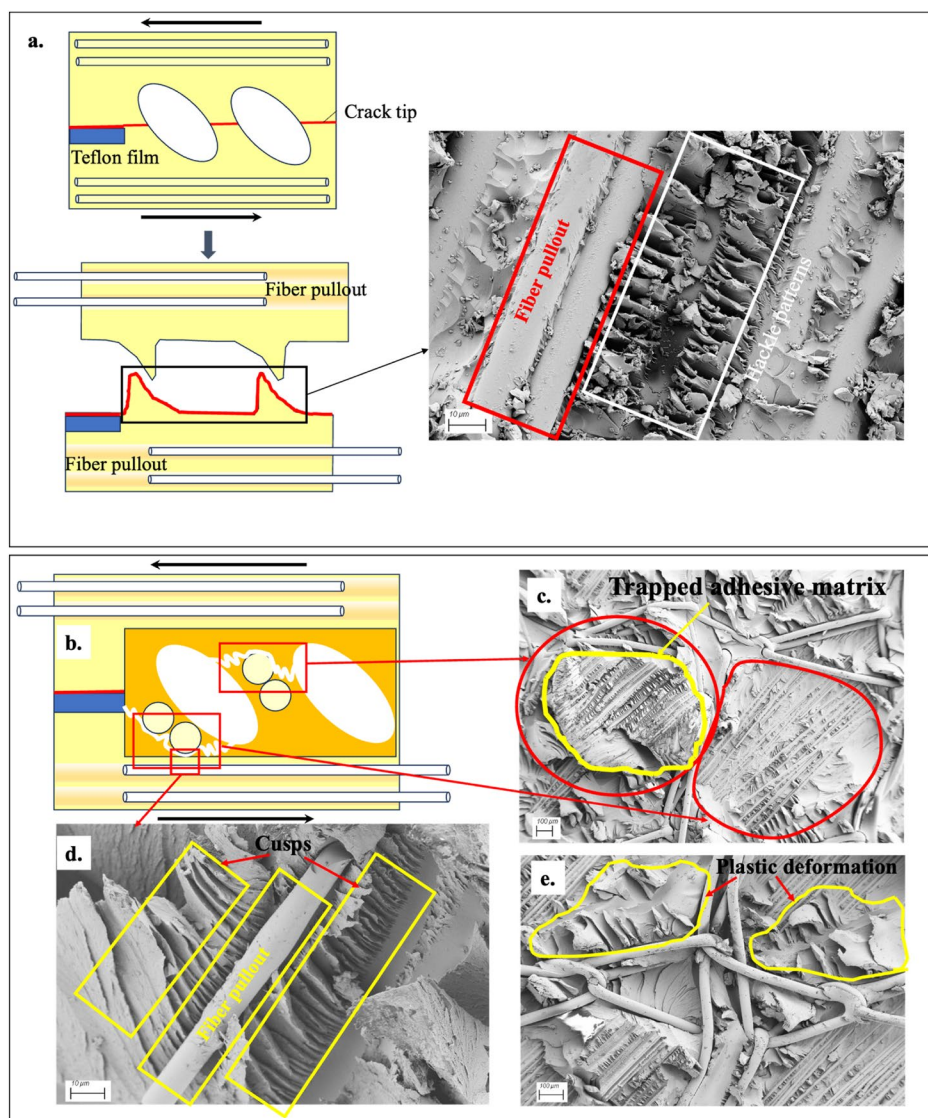
FIGURE 12 | SEM images of fracture surface under mode-II for (a) REF and (b–e) ALE samples, along with schematic representations of fracture mechanisms.
