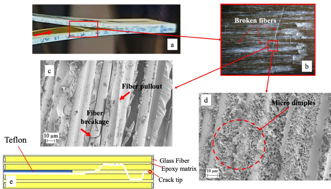
FIGURE 6 | Fractography of REF sample under Mode-I test.
