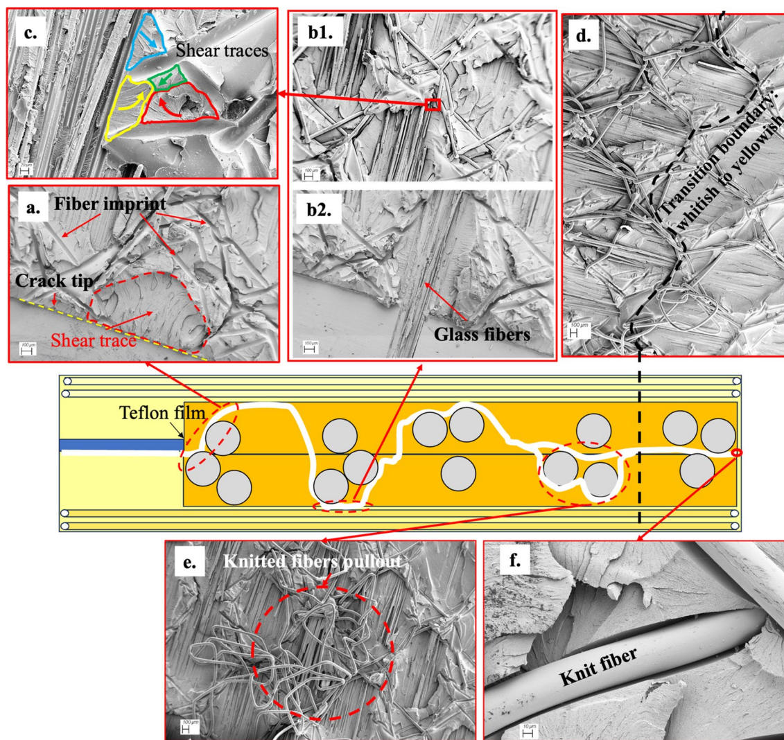
FIGURE 10 | Schematic representation of crack path and SEM images of the fracture phases for ALE sample under Mode-I test.
