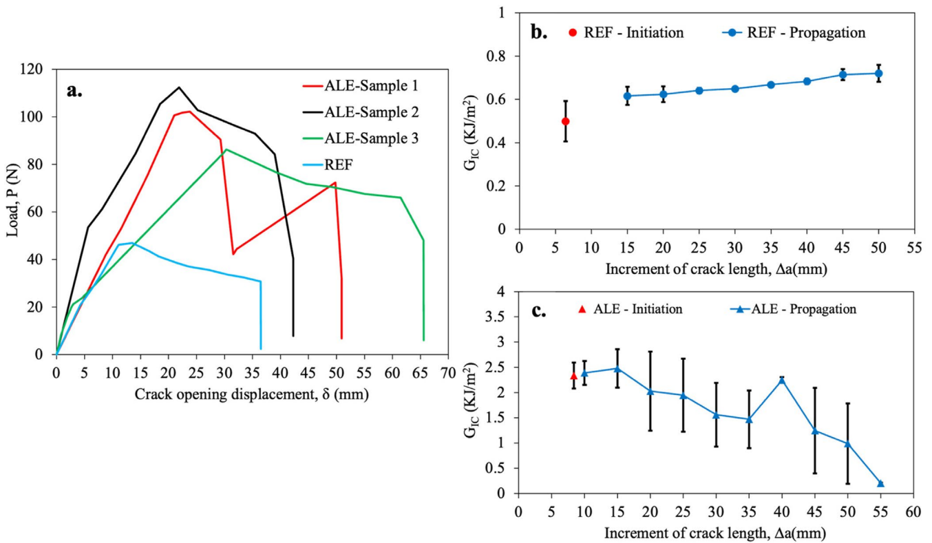
FIGURE 3 | (a) Load–displacement curves, and G_{IC} —crack length diagrams of DCB samples for (b) REF and (c) ALE samples.
