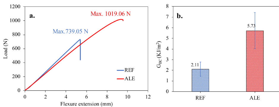
FIGURE 4 | (a) Load-flexure extension and (b) G_{IIC} diagrams of ENF samples for REF and ALE samples.
