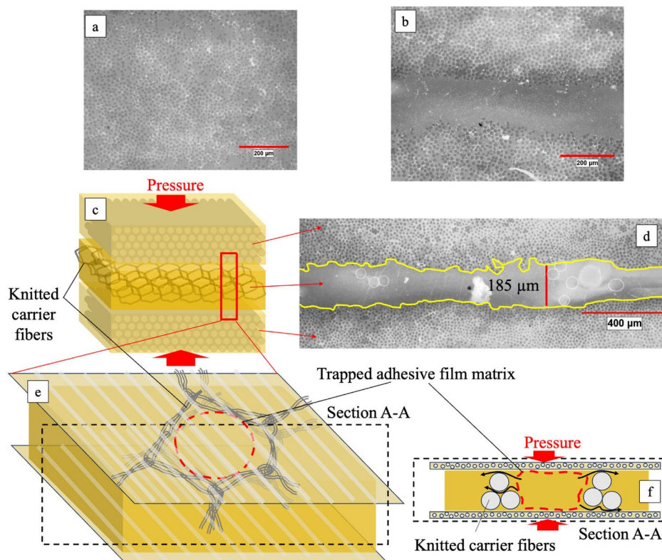
FIGURE 2 | Microscopic images of cross-sections showing (a) REF and (b) ALE samples; (c) a representative schematic of ALE samples; (d) variation in adhesive layer thickness and distribution of carrier fibers in ALE; (e) a magnified schematic representation of carrier fibers; and (f) the role of carrier fibers in controlling adhesive layer thickness under pressure.
