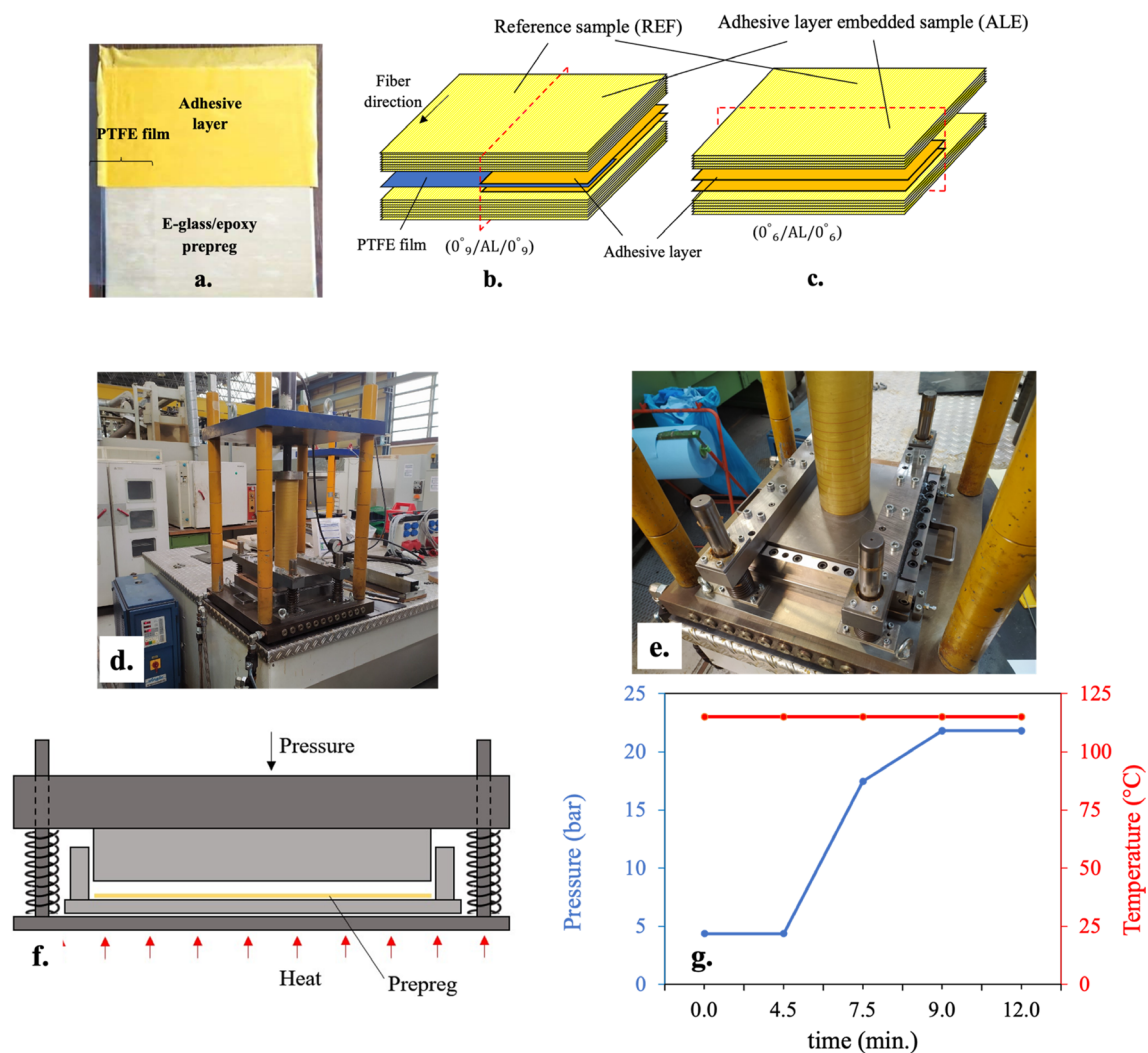
FIGURE 1 | Sample preparation with (a) placement of adhesive layer and PTFE film in laminate (top view), and laminate stacking sequences and schematics of adhesive layer position in half of composite sheets for (b) fracture sample and (c) tensile test sample, and sample manufacturing steps illustrating (d) hot press machine, (e) mold, (f) schematics of applied pressure and heat in mold, and (g) process parameters for pressure and temperature applied in hot press.
