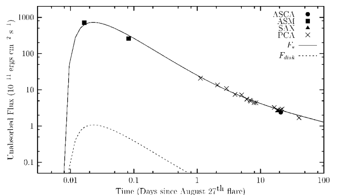
FIG. 3.—Same as Fig. 1, but for f = 0.9
