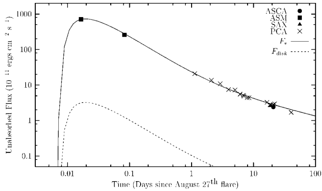
FIG. 1.—Data points ( RXTE/ASM , RXTE/PCA , BeppoSAX , and ASCA measurements) taken from Woods et al. (2001; see the text for the details and uncertainties of the measurements). The upper curve is the model flux from the surface of the neutron star, and the lower curve is the model disk flux. For this illustrative model (model 1), f \approx 0.1 . The parameters of models 1–3 are presented in Table 1.
