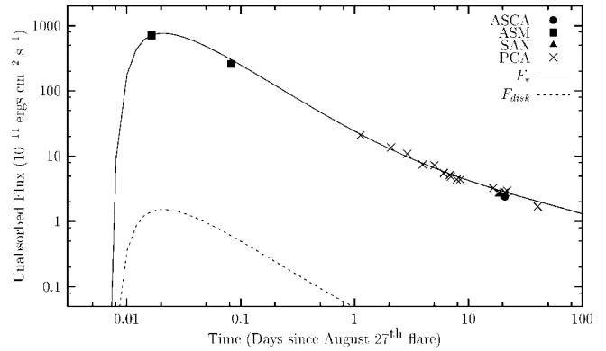
FIG. 2.—Same as Fig. 1, but for f = 0.5
