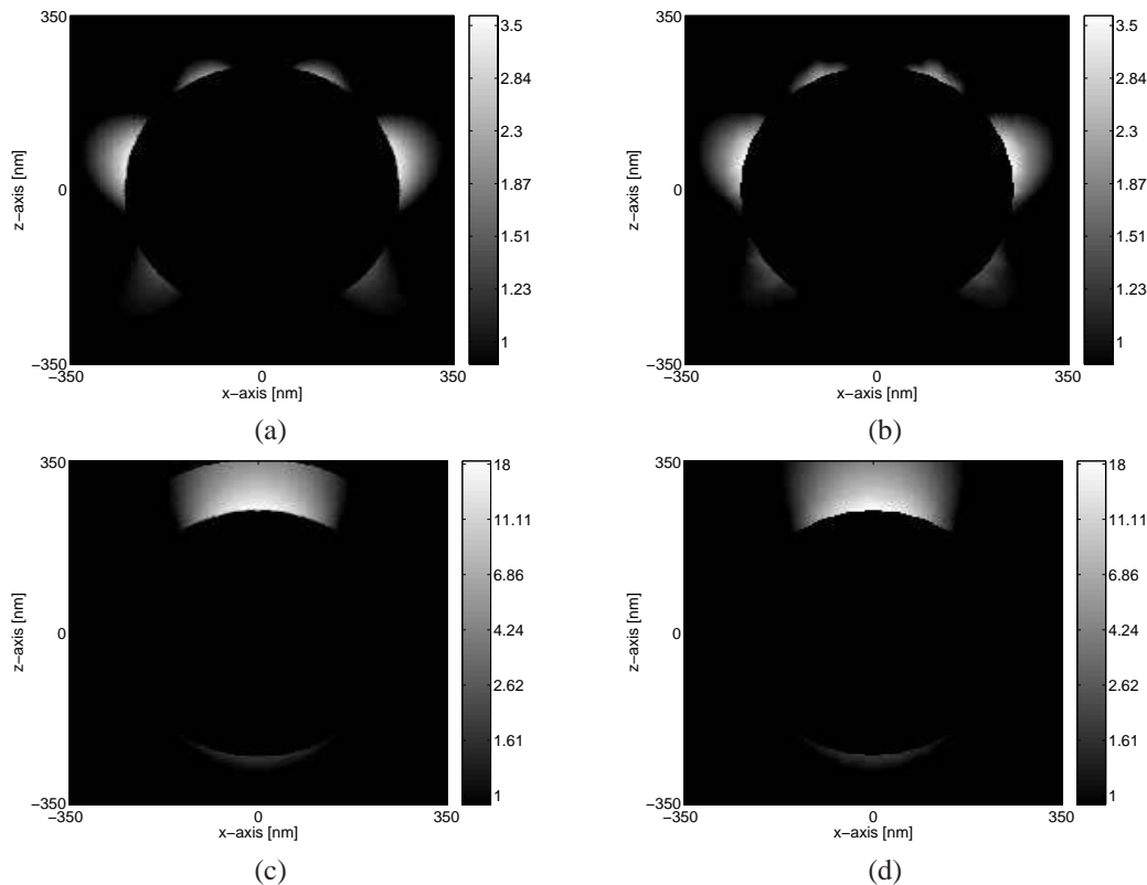
Fig. 6. Interaction of a radially polarized focused beam with a silver sphere with a 250 nm radius. The total electric field is plotted on the \hat{x} - \hat{z} plane. (a) Solution using Mie series for |E_x(x,y)|^2 , (b) FEM solution for |E_x(x,y)|^2 , (c) Solution using Mie series for |E_z(x,y)|^2 , (d) FEM solution for |E_z(x,y)|^2 . |E_y(x,y)|^2 components for both solutions are negligible.
