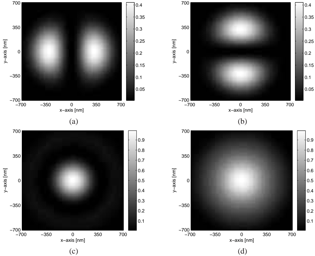
Fig. 2. Various electric fields components for the radially polarized focused beam at the focal plane. The results are normalized with the maximum value of the total electric field. (a) E_x(x,y) , (b) E_y(x,y) , (c) E_z(x,y) , and (d) E_t(x,y) .
