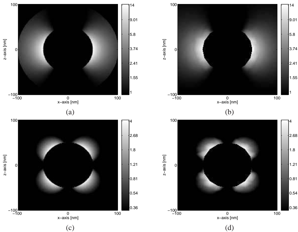
Fig. 5. Interaction of a linearly polarized focused beam with a silver sphere with a 50 nm radius. The total electric field is plotted on the \hat{x}\hat{z} plane. (a) Solution using Mie series for |E_x(x,y)|^2 , (b) FEM solution for |E_x(x,y)|^2 , (c) Solution using Mie series for |E_z(x,y)|^2 , (d) FEM solution for |E_z(x,y)|^2 . |E_y(x,y)|^2 components for both solutions are negligible.
