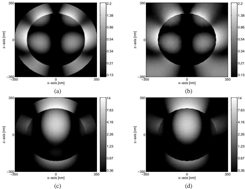
Fig. 8. Interaction of a radially polarized focused beam with a dielectric sphere with a 250 nm radius. Dielectric index of the sphere is 2. The total electric field is plotted on the \hat{x} - \hat{z} plane. (a) Solution using Mie series for |E_x(x,y)|^2 , (b) FEM solution for |E_x(x,y)|^2 , (c) Solution using Mie series for |E_z(x,y)|^2 , (d) FEM solution for |E_z(x,y)|^2 . |E_y(x,y)|^2 components for both solutions are negligible.
