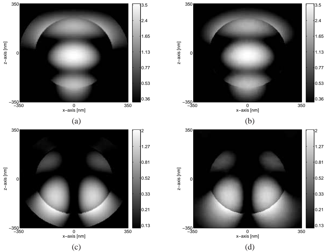
Fig. 9. Interaction of a linearly polarized focused beam with a dielectric sphere with a 250 nm radius. Dielectric index of the sphere is 2. The total electric field is plotted on the \hat{x} - \hat{z} plane. (a) Solution using Mie series for |E_x(x,y)|^2 , (b) FEM solution for |E_x(x,y)|^2 , (c) Solution using Mie series for |E_z(x,y)|^2 , (d) FEM solution for |E_z(x,y)|^2 . |E_y(x,y)|^2 components for both solutions are negligible.
