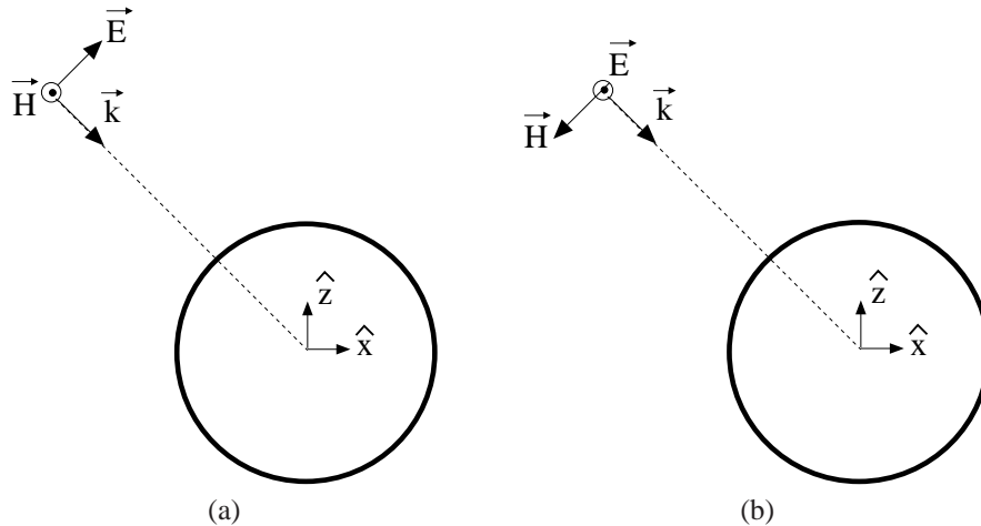
Fig. 3. Spherical particle illuminated by (a) TM polarized plane wave, and (b) TE polarized plane wave.
