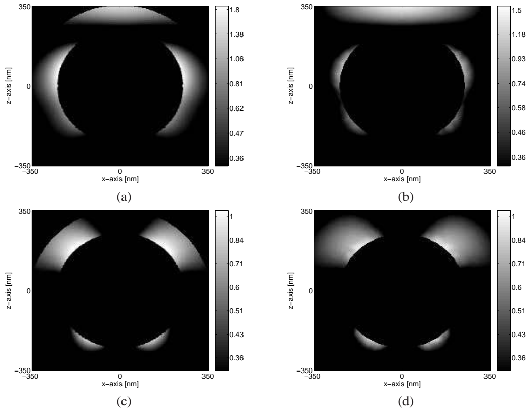
Fig. 7. Interaction of a linearly polarized focused beam with a silver sphere with a 250 nm radius. The total electric field is plotted on the \hat{x} - \hat{z} plane. (a) Solution using Mie series for |E_x(x,y)|^2 , (b) FEM solution for |E_x(x,y)|^2 , (c) Solution using Mie series for |E_z(x,y)|^2 , (d) FEM solution for |E_z(x,y)|^2 . |E_y(x,y)|^2 components for both solutions are negligible.
