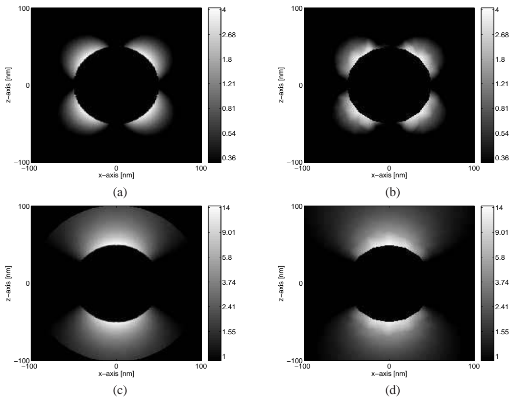
Fig. 4. Interaction of a radially polarized focused beam with a silver sphere with a 50 nm radius. The total electric field is plotted on the \hat{x} - \hat{z} plane. (a) Solution using Mie series for |E_x(x,y)|^2 , (b) FEM solution for |E_x(x,y)|^2 , (c) Solution using Mie series for |E_z(x,y)|^2 , (d) FEM solution for |E_z(x,y)|^2 . |E_y(x,y)|^2 components for both solutions are negligible.
