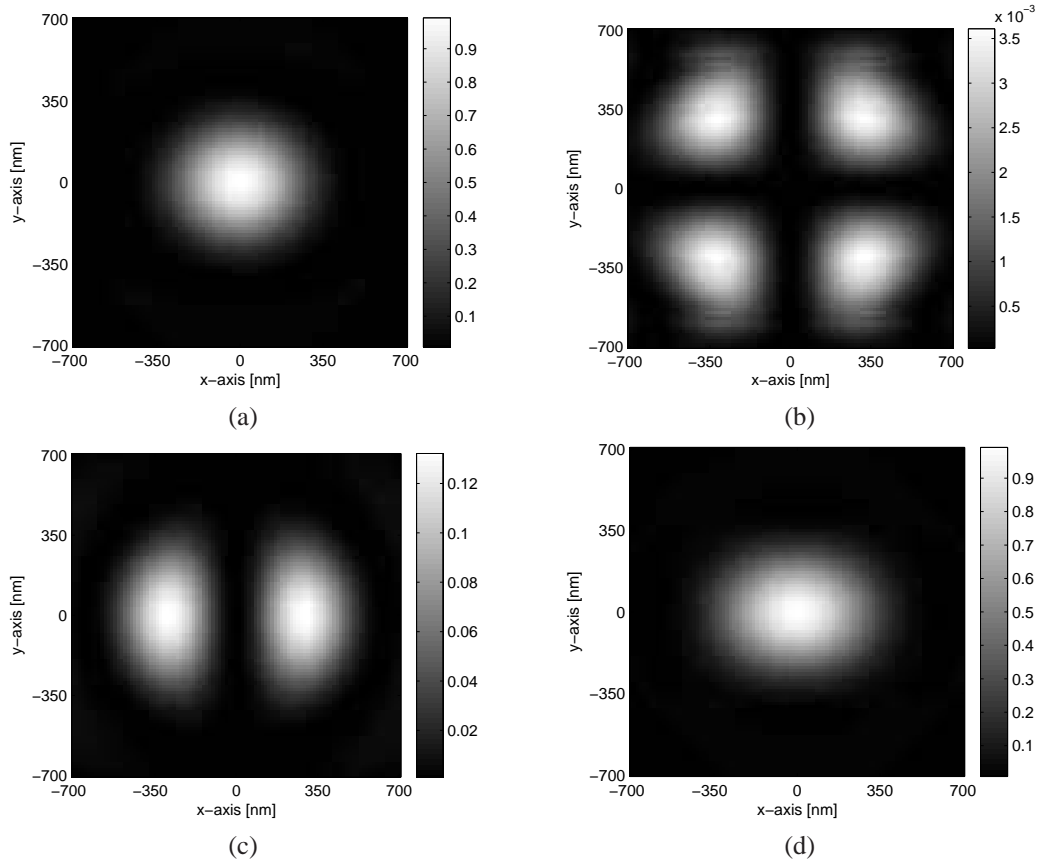
Fig. 1. Various electric fields components for the linearly polarized focused beam at the focal plane. The results are normalized with the maximum value of the total electric field. (a) E_x(x, y) , (b) E_y(x, y) , (c) E_z(x, y) , and (d) E_t(x, y) .
