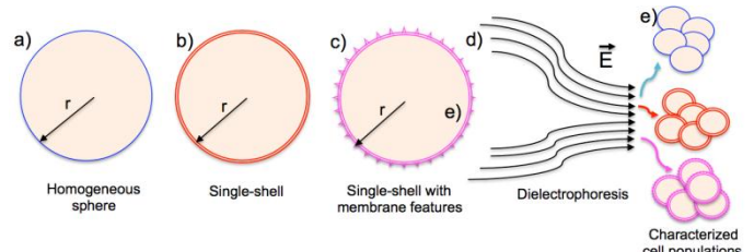
Fig. 1. Dielectric shell models for cells. a) Homogeneous sphere model, b) Single-shell model, shell thickness equals to cellular membrane thickness, c) Single-shell model with membrane features such as microvilli, filopodia, ruffles and folds, d) Applied nonuniform electric field ( E ), e) characterized subpopulations of cells due to their membrane differences
