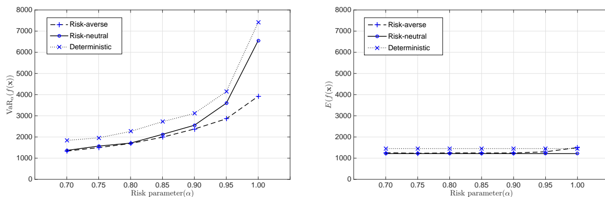
Figure 1: The effect of the risk parameter \alpha on the VaR and the expectation of f(\mathbf{x}) .
