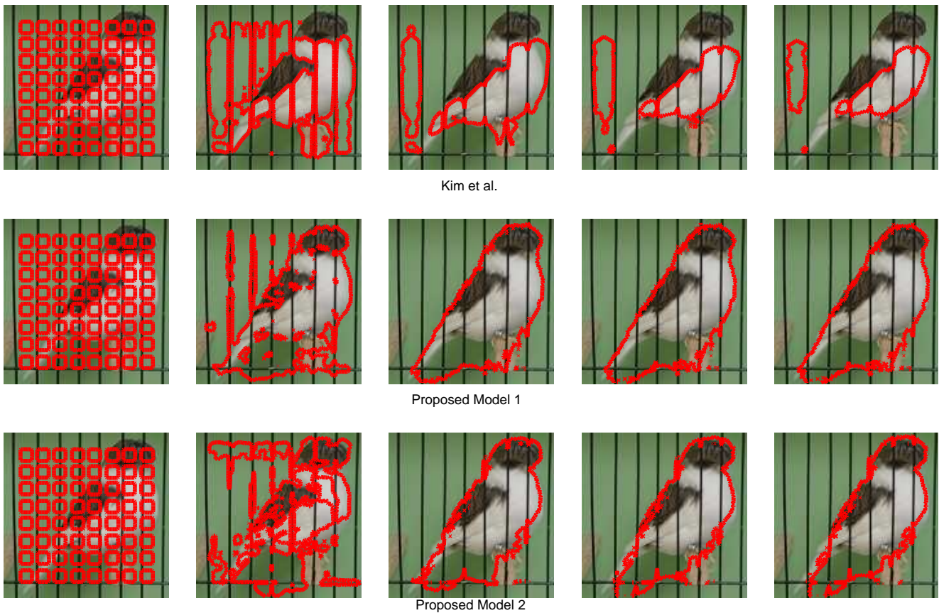
Fig. 9 Segmentation of a bird. First row shows the segmentation result of [12]. Second row shows the segmentation result of proposed model 1. Third row shows the result of proposed model 2. Leftmost and rightmost columns show the initial curve and the final segmentation result, respectively, whereas the middle columns show intermediate states in the curve evolution process.
