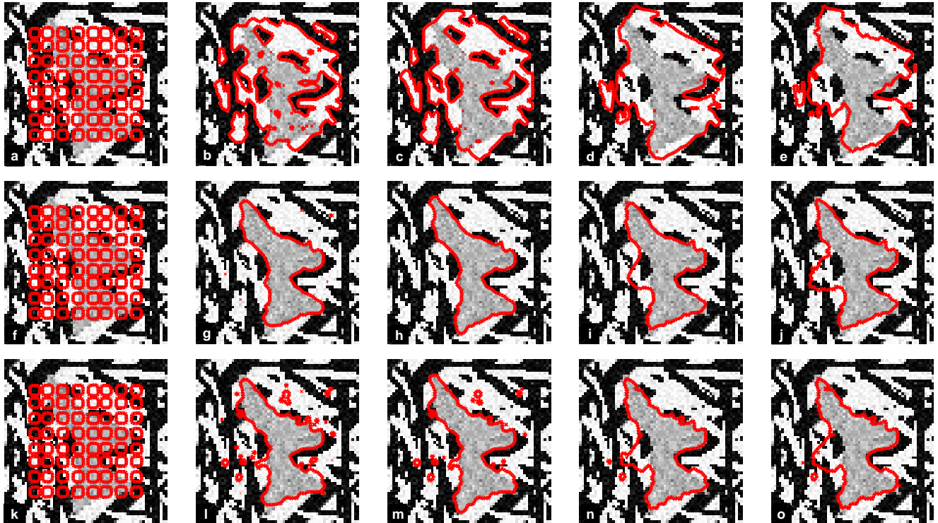
Fig. 3 Segmentation of the aircraft image. First row (a-e) shows the segmentation result of [12]. Second row (f-j) shows the segmentation result of proposed model 1 which is based on learning and using the foreground and the background intensity distributions. Third row (k-o) shows the result of proposed model 2 in which the background is treated as uniformly distributed. Leftmost and rightmost columns show the initial curve and the final segmentation result, respectively, whereas the middle columns show intermediate states in the curve evolution process.
