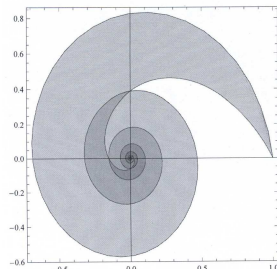
FIGURE 2. Essential Spectra of C_\varphi for a = 5 and b = 25
