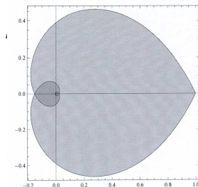
FIGURE 1. Essential Spectra of C_\varphi for a = -5 and b = 5
