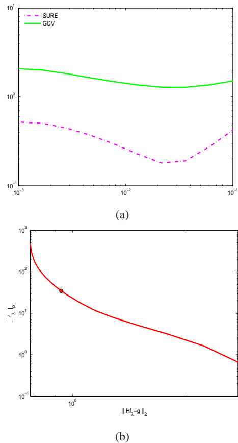
Fig. 10. (a) SURE and GCV curves, (b) L-curve and corresponding L-corner for the backhoe scene when p = 1 and SNR=10 dB.
