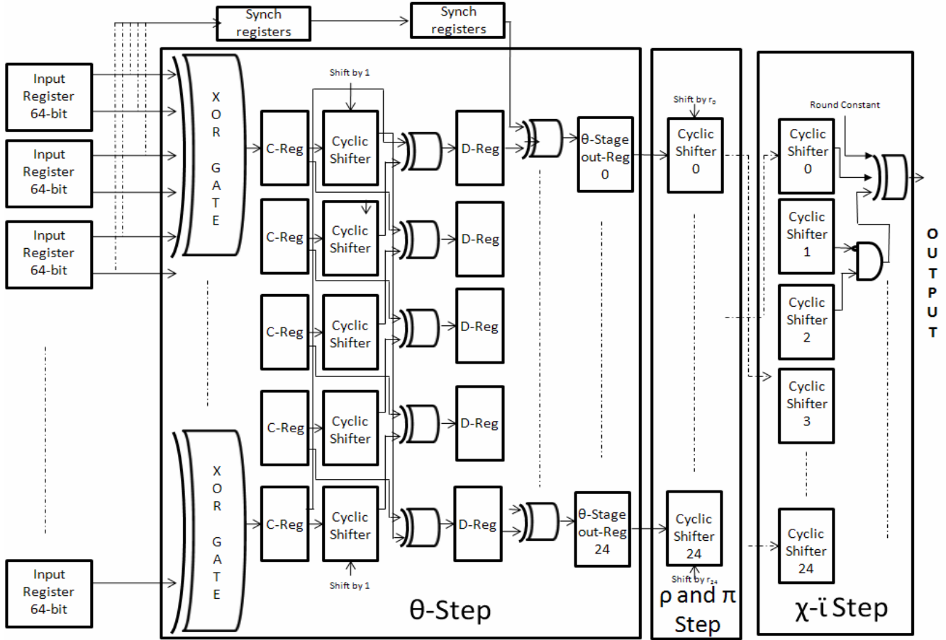
Figure 8. Block Diagram of Keccak Hardware
