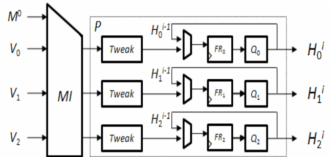
Figure 9. Block Diagram of the Luffa Hardware Architecture
