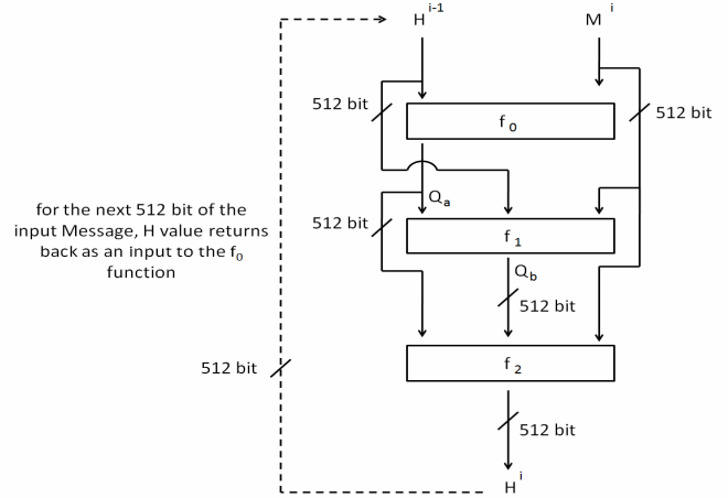
Figure 10. Block Diagram of the BMW Hardware Architecture
