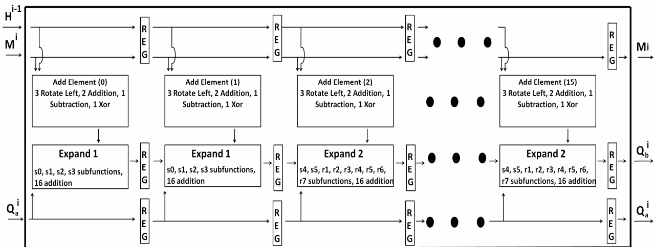
Figure 12. Hardware Architecture of Pipelined f_1 function
