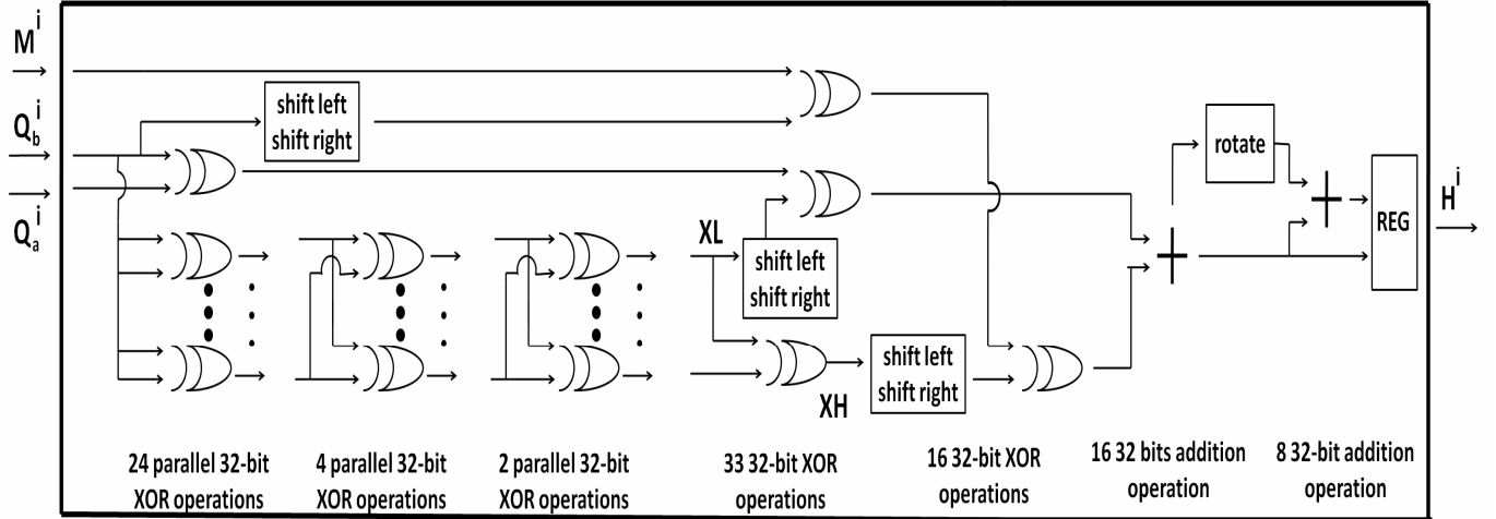
Figure 13. Hardware Architecture of f_2 function
