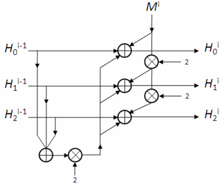
Figure 3. Block diagram of the Message Injection module
