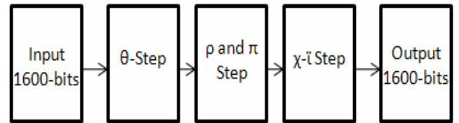
Figure 6. High-Level Pipeline Stages of Keccak Hardware
