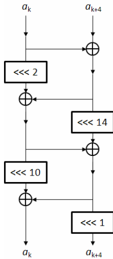
Figure 5. Block diagram of MixWord function
