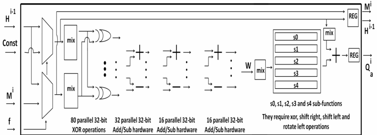
Figure 11. Hardware Architecture of f_0 function
