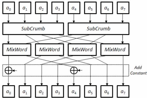
Figure 4. Block diagram of the Step module
