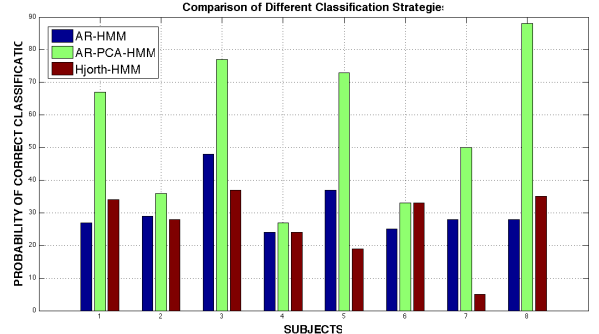
Fig. 2: Performance of the proposed AR-PCA-HMM approach as compared to other HMM-based techniques.
