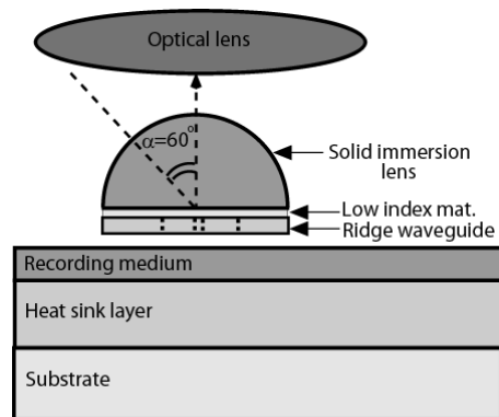
Figure 1. A schematic illustration of an optical transducer, which is placed at the end of an optical lens system, is given. The optical transducer is placed in the vicinity of a near-field sample, which is the recording magnetic medium for HAMR.
