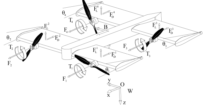
Fig. 3. Aerial Vehicle in Horizontal Flight Configuration
